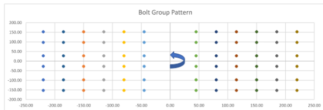
Figure 4. Splice connection design for the rivet ("bolt") group – incorporating polar moment of inertia
