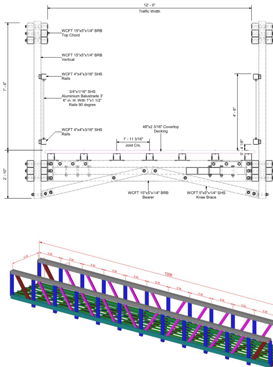
Figure 1. 100ft Bridge Geometry (Cross-section and Elevation view)
